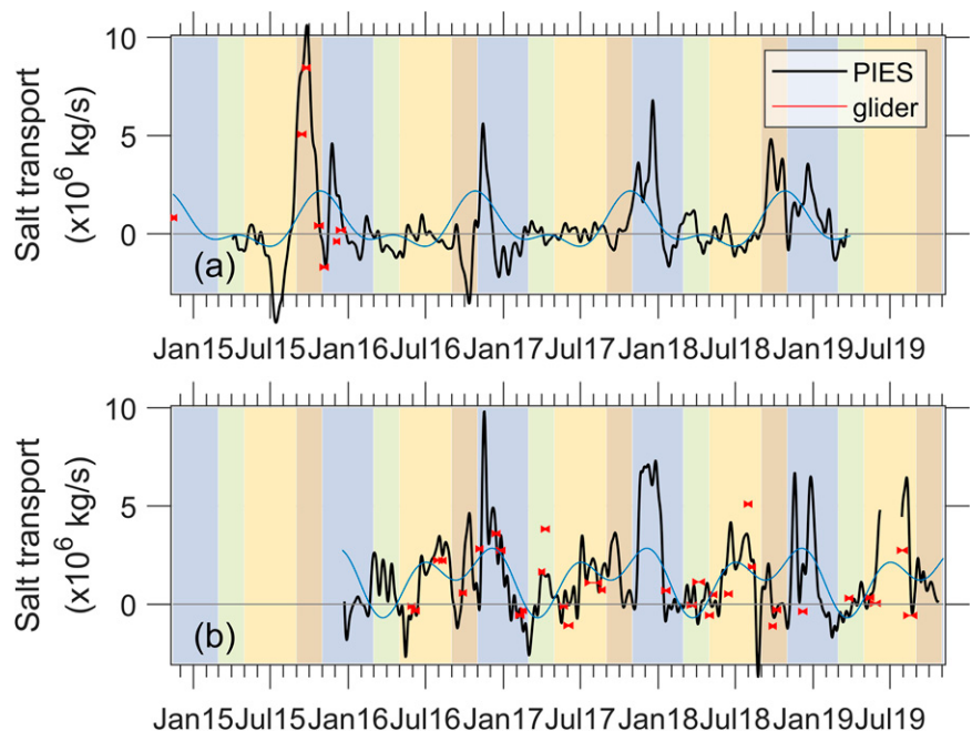
FIG. 6. Estimated eddy salt flux across the Sri Lankan (a) eastern and (b) southern sections. Values in (a) are computed from section-depth velocity and salinity, whereas values in (b) are computed from section-mean velocity and salinity. Glider results are shown in red, and results from PIES, satellite altimetry, and SMAP SSS are shown in black. The lengths of the red symbols represent the time it took the glider to complete the crossing bracketed by the PIES. The seasonal cycles, constructed as the sums of the annual and semiannual harmonics, are plotted in blue. Background shading denotes monsoon seasons as in Fig. 4.
